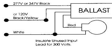
Wiring Diagram 34
