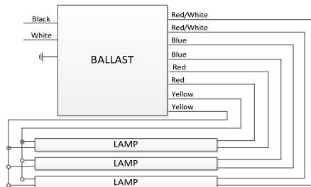
Three Lamp Application
