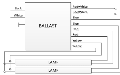
Cap unused red/white leads, insulate to 600 Volts Two Lamp Application
